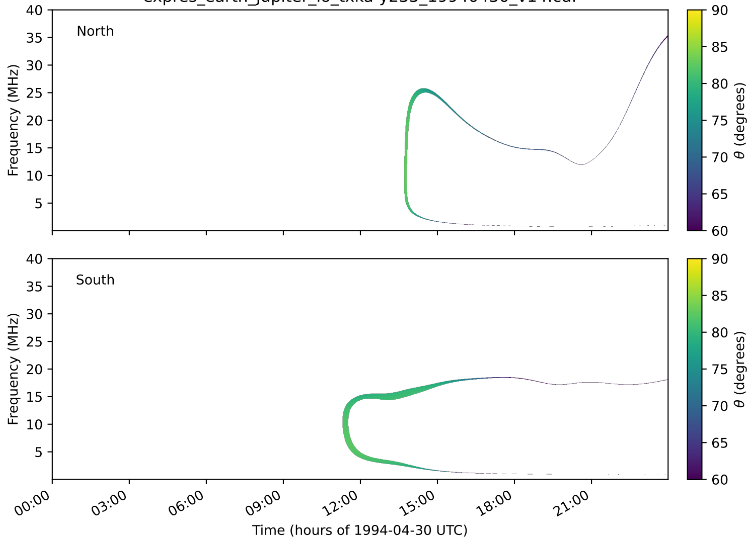
expres_earth_jupiter_io_txka-y235_19940430_v14.cdf
