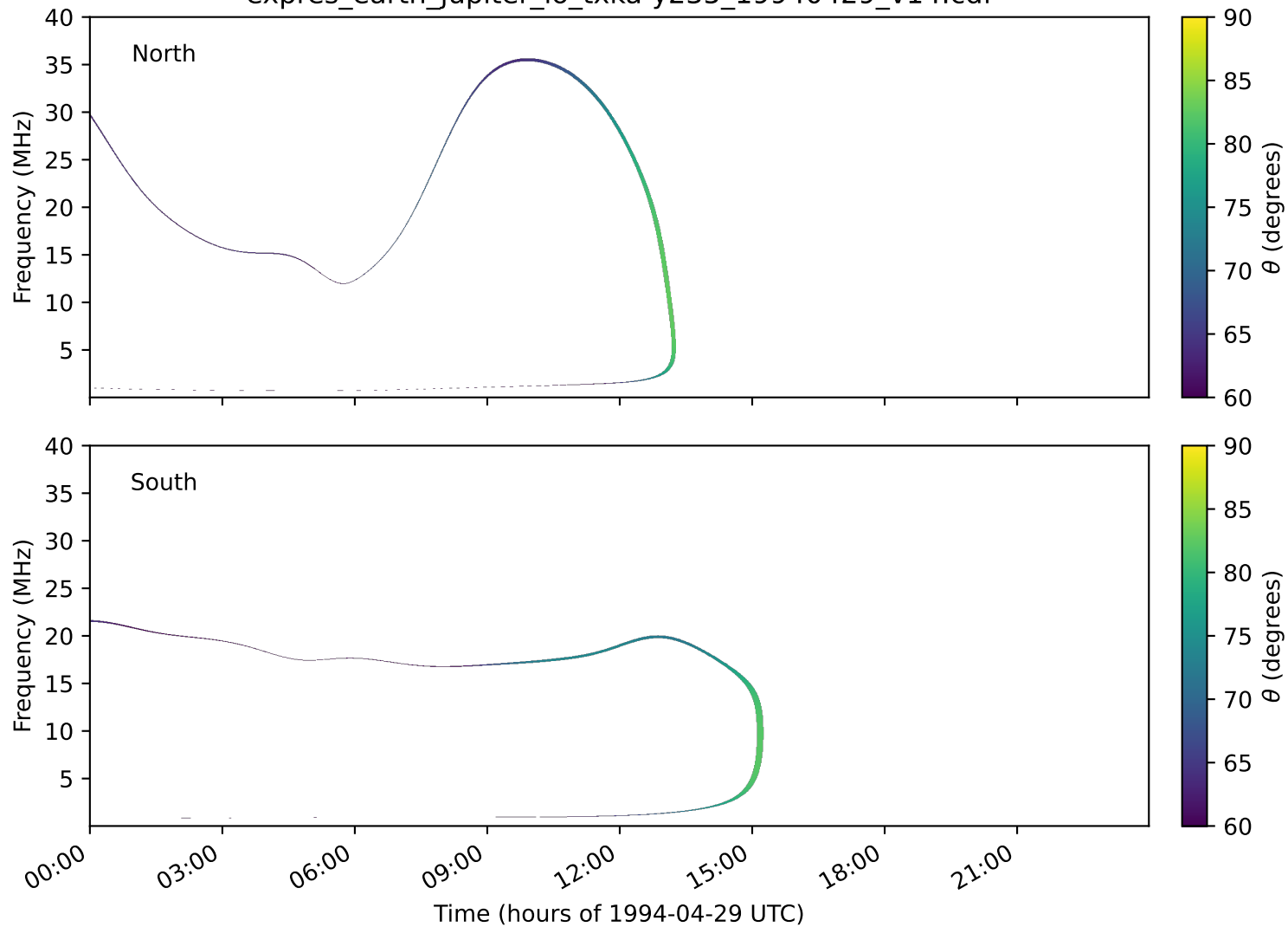
expres_earth_jupiter_io_txka-y235_19940429_v14.cdf
