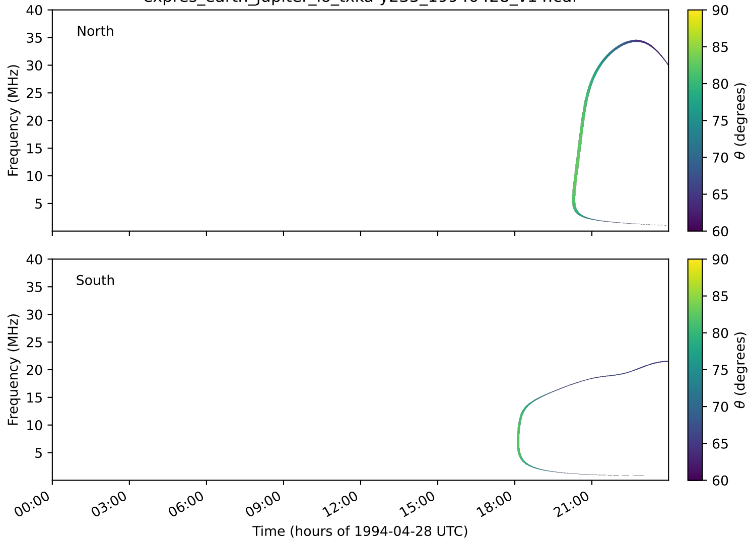
expres_earth_jupiter_io_txka-y235_19940428_v14.cdf
