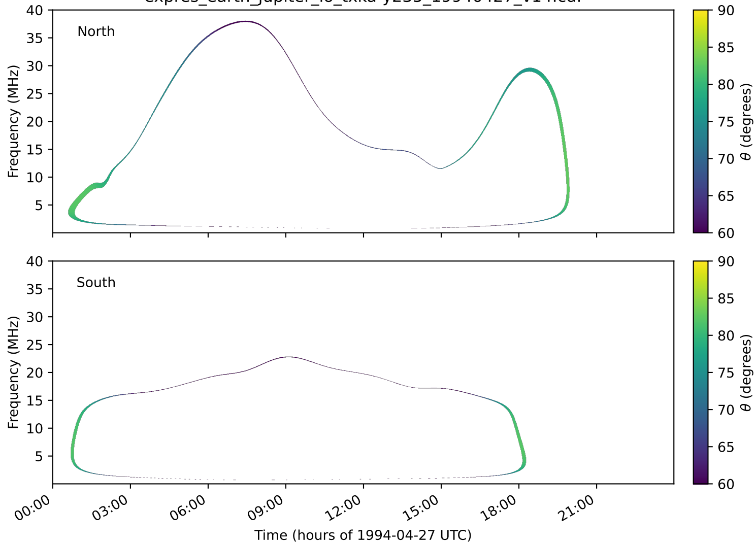
expres_earth_jupiter_io_txka-y235_19940427_v14.cdf
