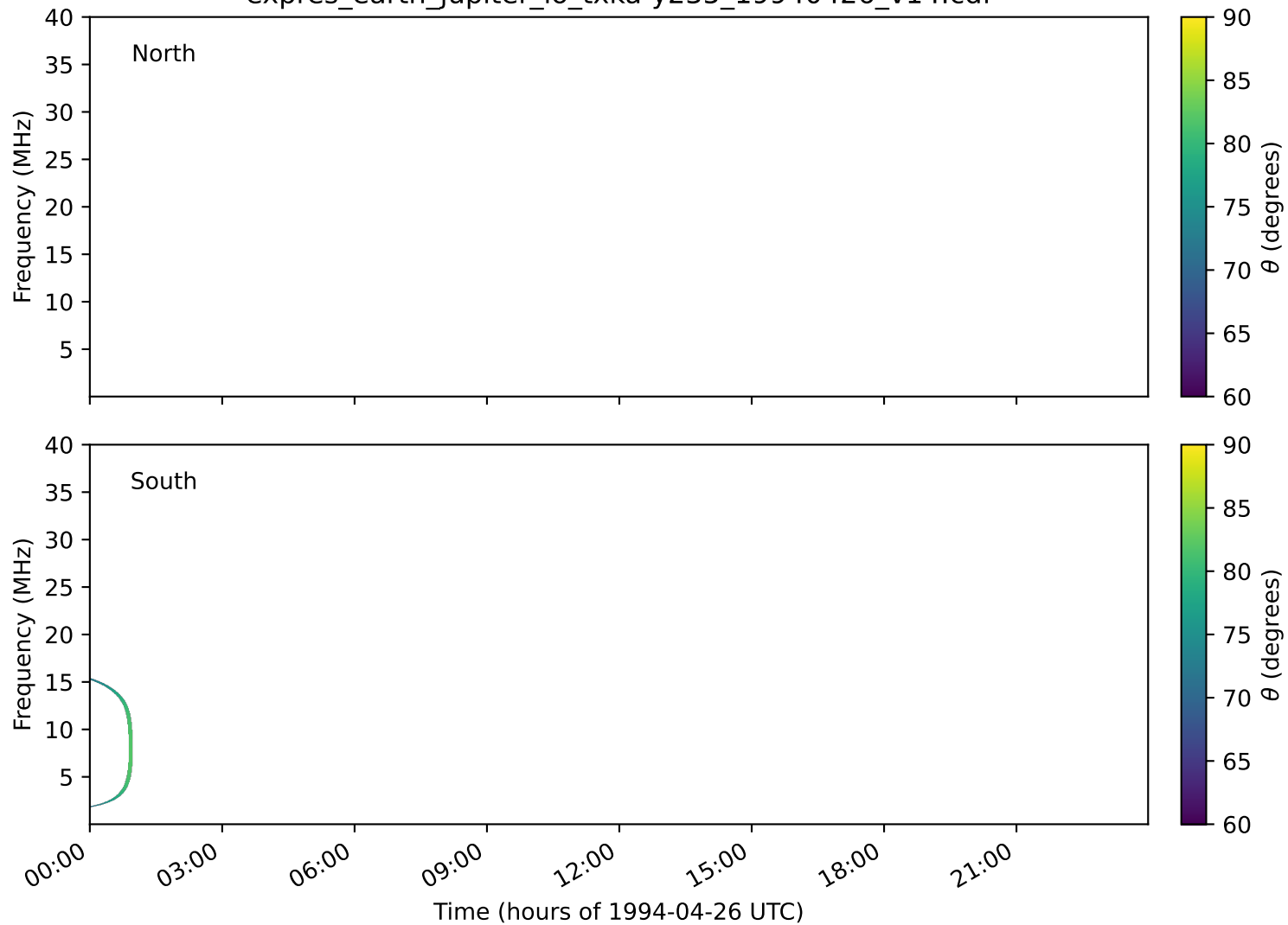
expres_earth_jupiter_io_txka-y235_19940426_v14.cdf
