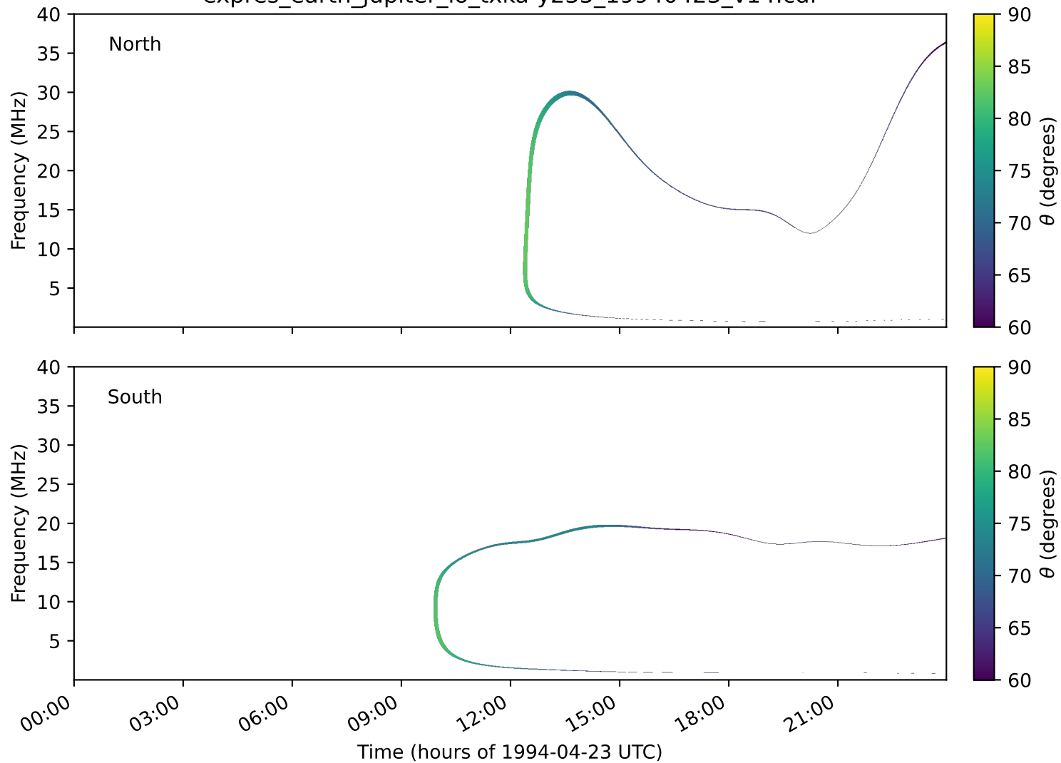
expres_earth_jupiter_io_txka-y235_19940423_v14.cdf
