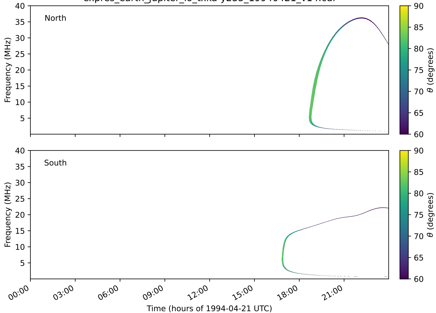
expres_earth_jupiter_io_txka-y235_19940421_v14.cdf
