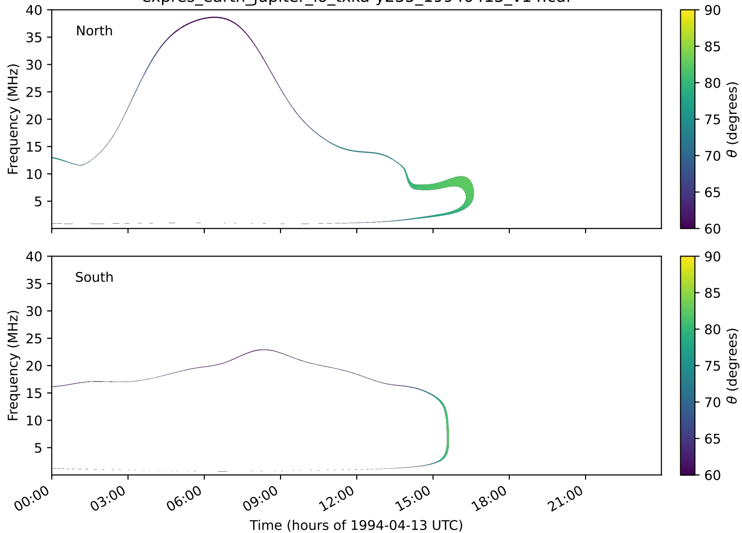
expres_earth_jupiter_io_txka-y235_19940413_v14.cdf
