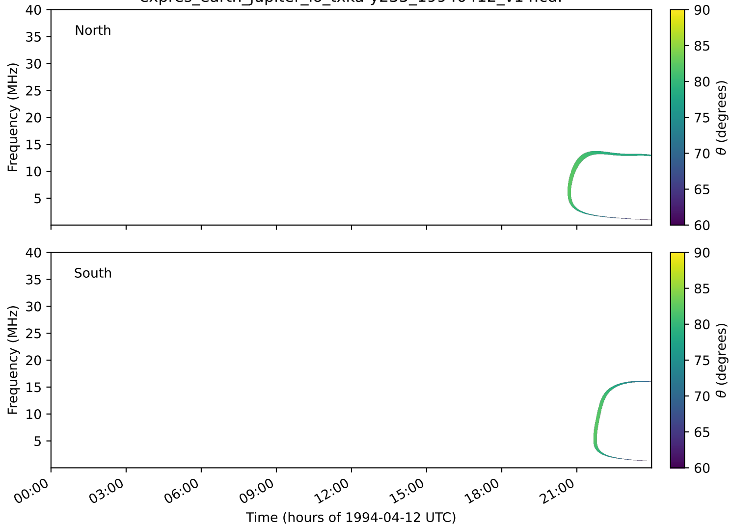
expres_earth_jupiter_io_txka-y235_19940412_v14.cdf
