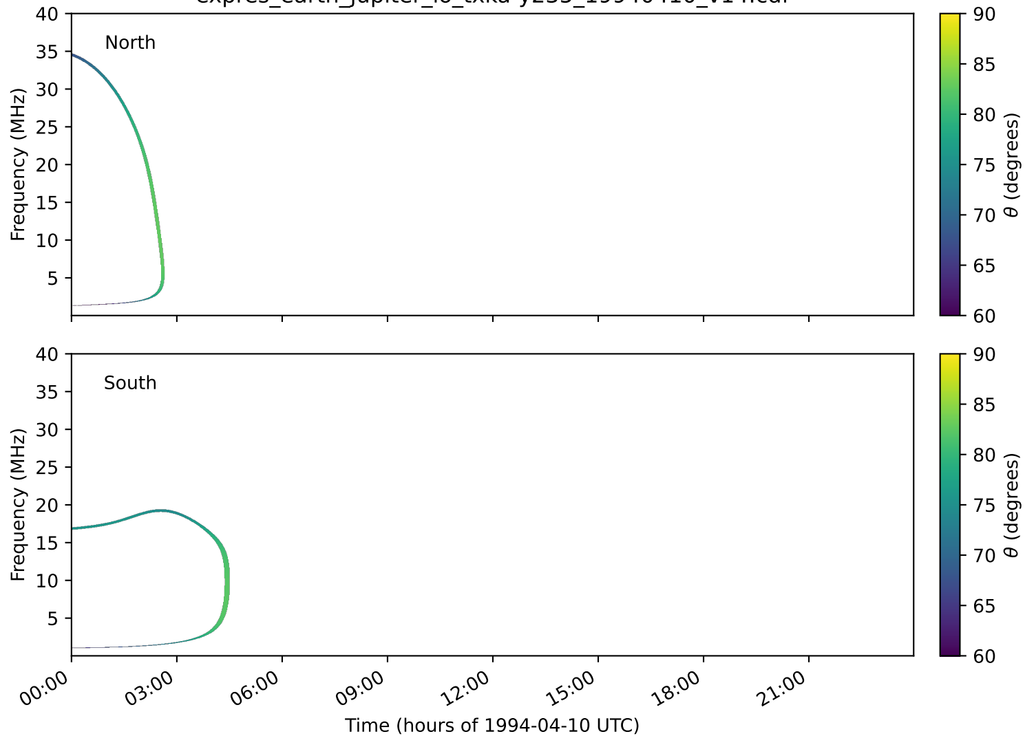
expres_earth_jupiter_io_txka-y235_19940410_v14.cdf
