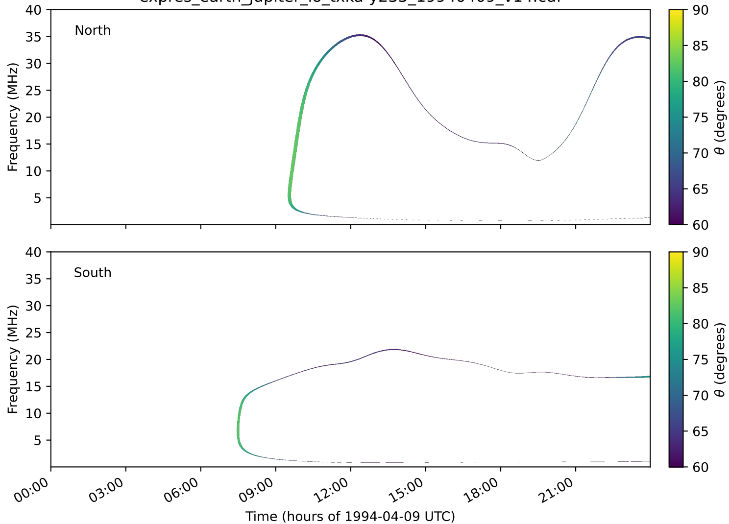
expres_earth_jupiter_io_txka-y235_19940409_v14.cdf
