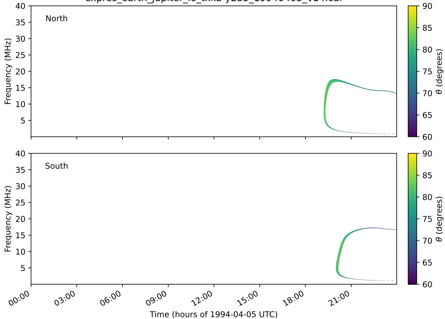
expres_earth_jupiter_io_txka-y235_19940405_v14.cdf
