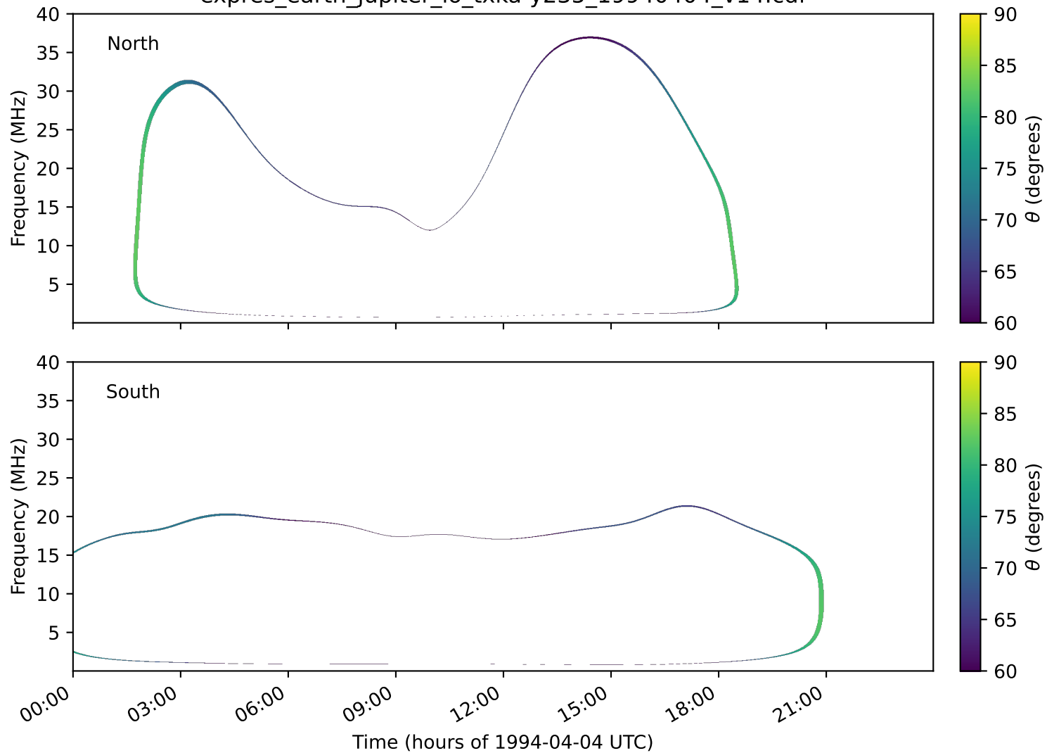
expres_earth_jupiter_io_txka-y235_19940404_v14.cdf
