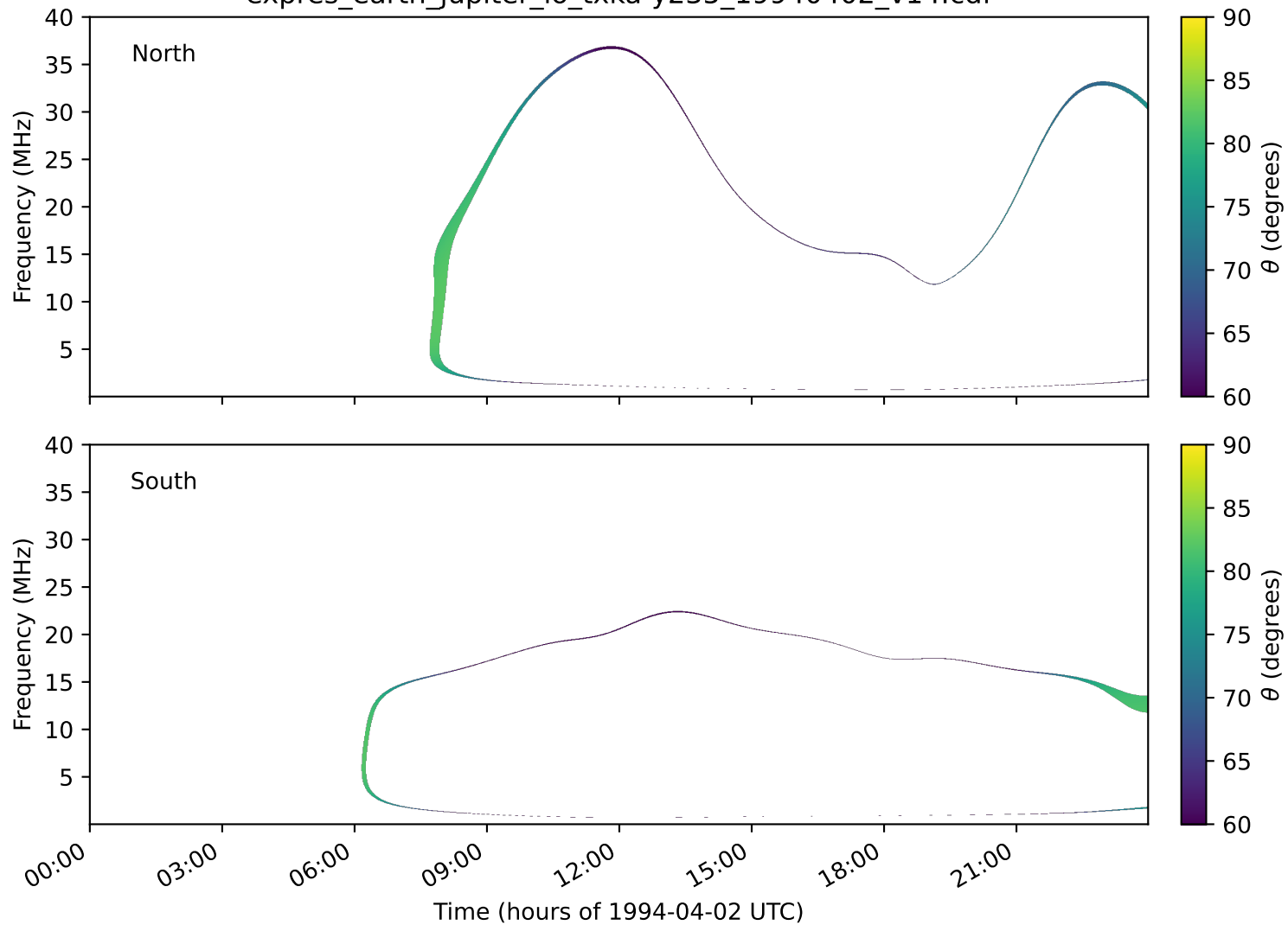
expres_earth_jupiter_io_txka-y235_19940402_v14.cdf
