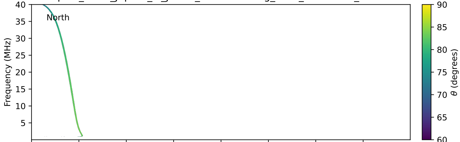
expres_earth_jupiter_io_jrm33_lossc-wid1deg_3kev_19940410_v11.cdf
