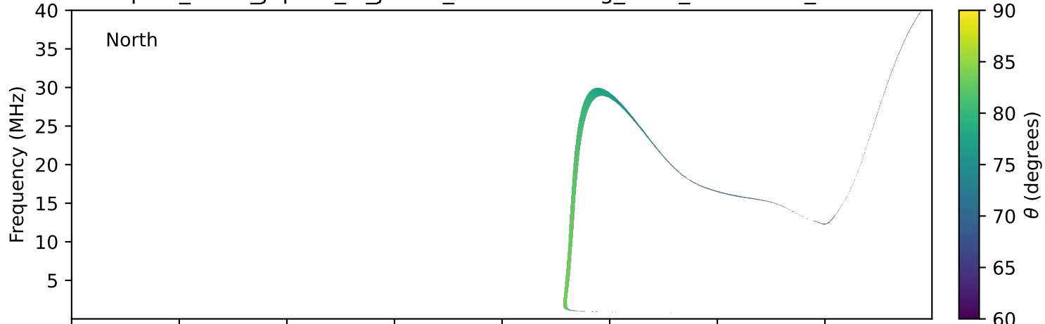
expres_earth_jupiter_io_jrm09_lossc-wid1deg_3kev_19940430_v11.cdf
