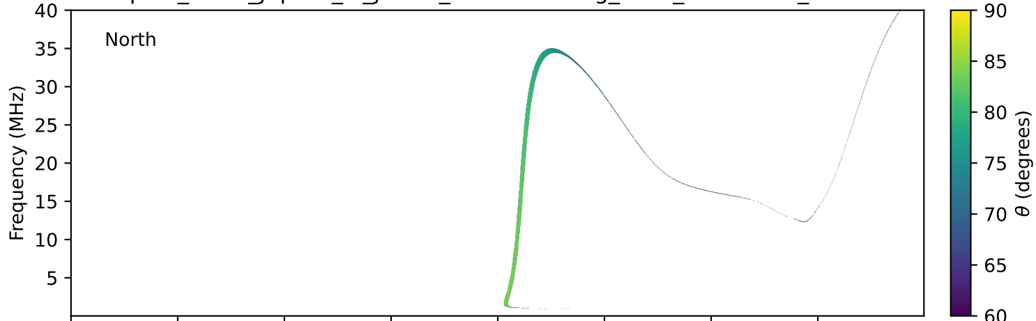
expres_earth_jupiter_io_jrm09_lossc-wid1deg_3kev_19940423_v11.cdf
