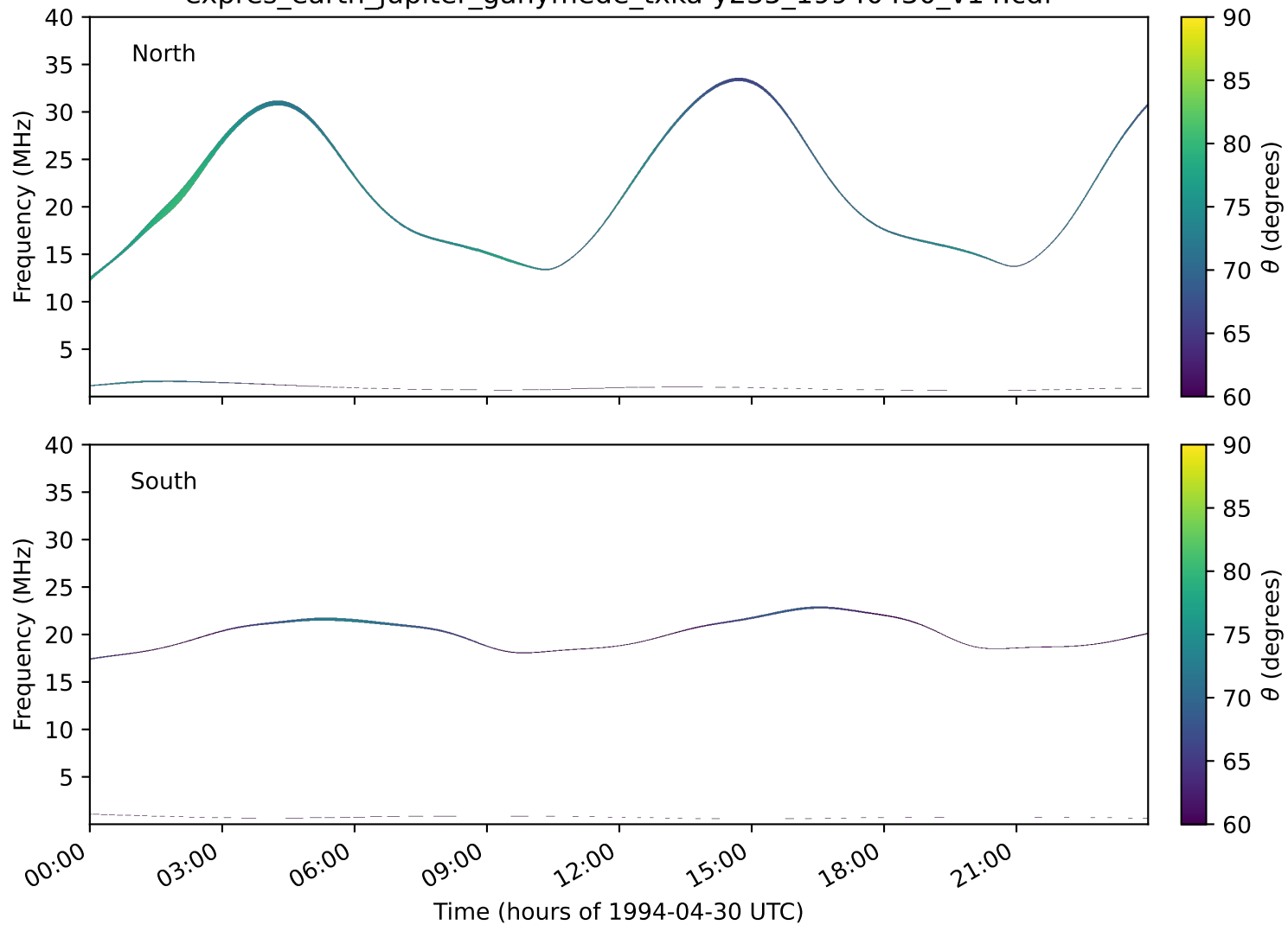
expres_earth_jupiter_ganymede_txka-y235_19940430_v14.cdf
