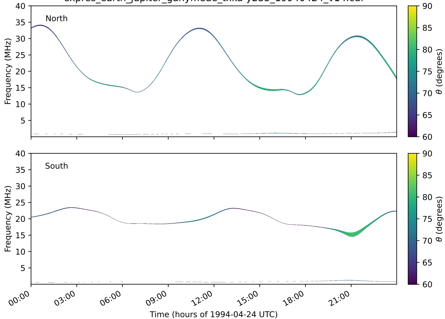
expres_earth_jupiter_ganymede_txka-y235_19940424_v14.cdf
