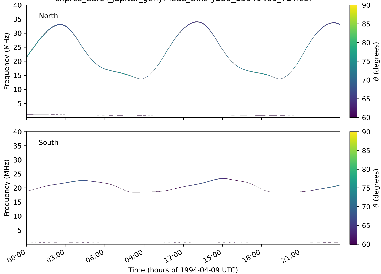
expres_earth_jupiter_ganymede_txka-y235_19940409_v14.cdf
