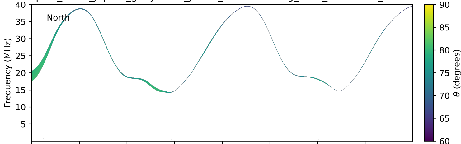
expres_earth_jupiter_ganymede_jrm33_lossc-wid1deg_3kev_19940416_v11.cdf
