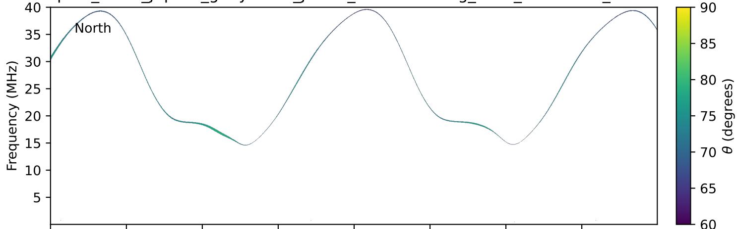
expres_earth_jupiter_ganymede_jrm33_lossc-wid1deg_3kev_19940402_v11.cdf
