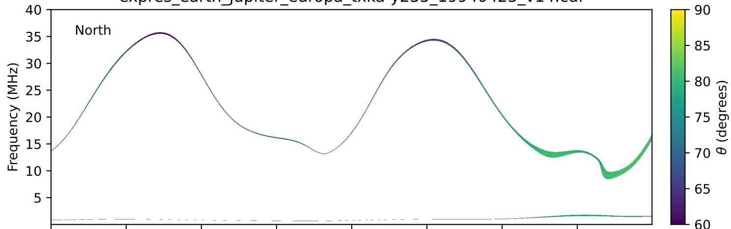
expres_earth_jupiter_europa_txka-y235_19940423_v14.cdf
