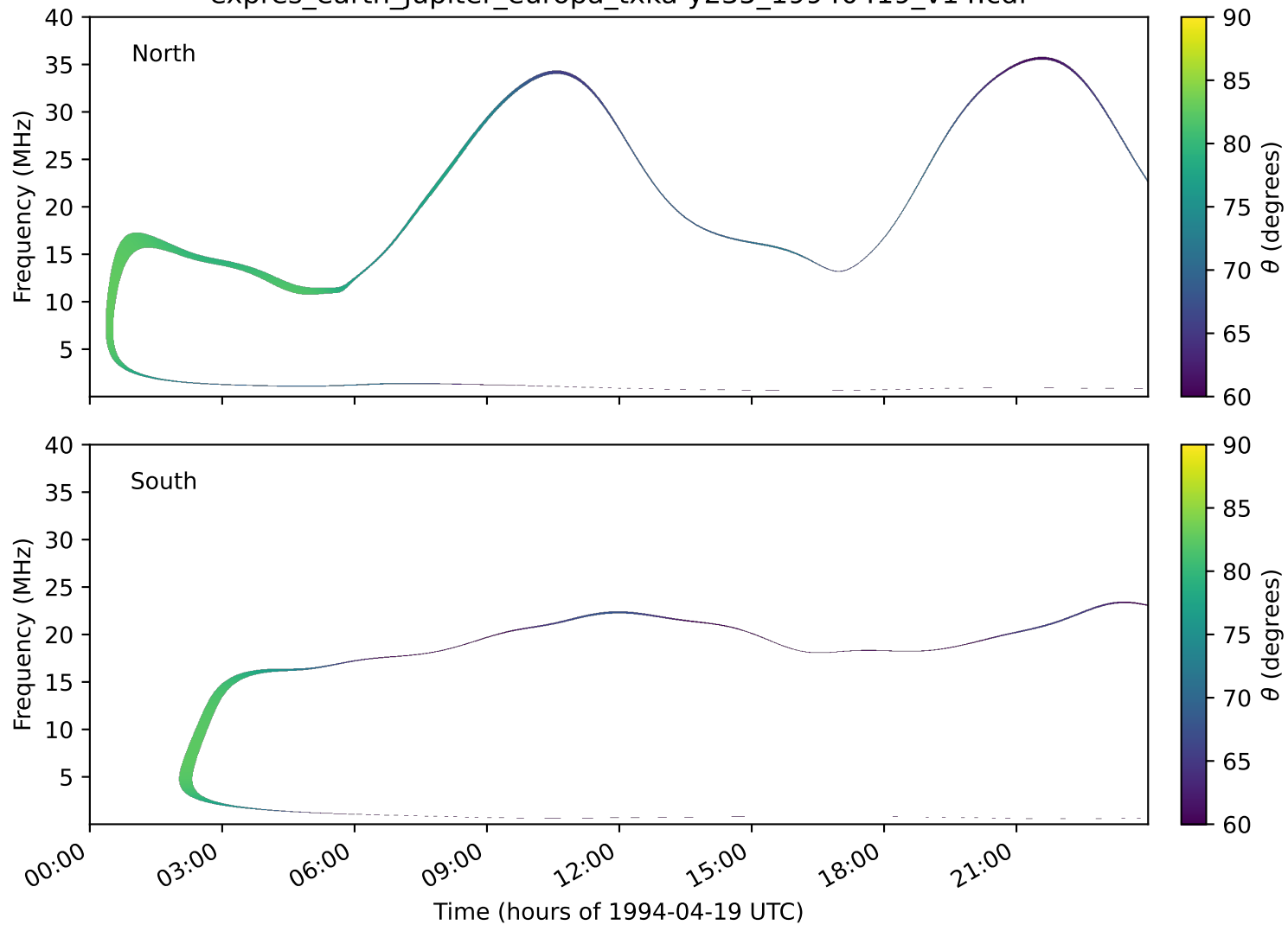
expres_earth_jupiter_europa_txka-y235_19940419_v14.cdf
