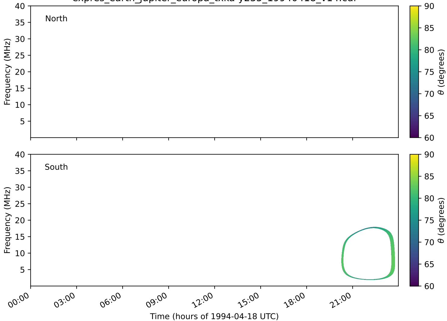
expres_earth_jupiter_europa_txka-y235_19940418_v14.cdf
