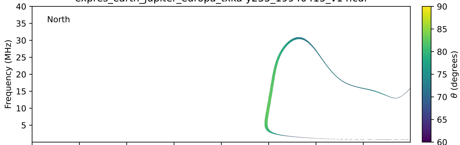
expres_earth_jupiter_europa_txka-y235_19940415_v14.cdf
