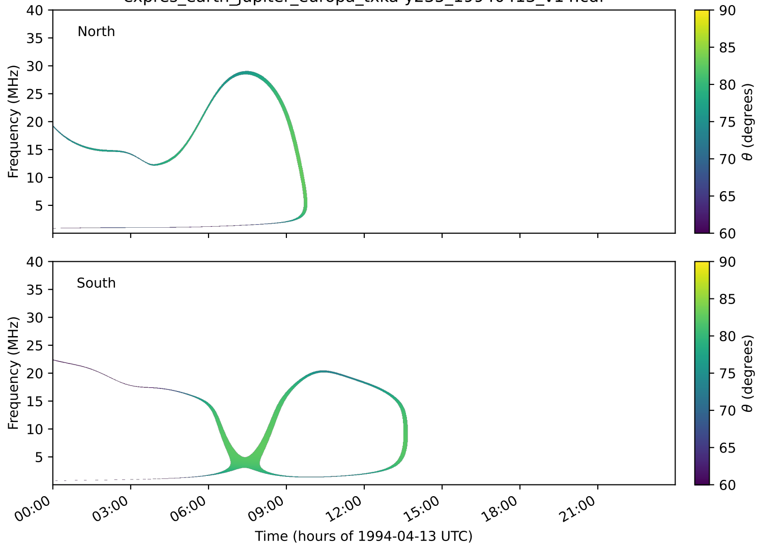
expres_earth_jupiter_europa_txka-y235_19940413_v14.cdf
