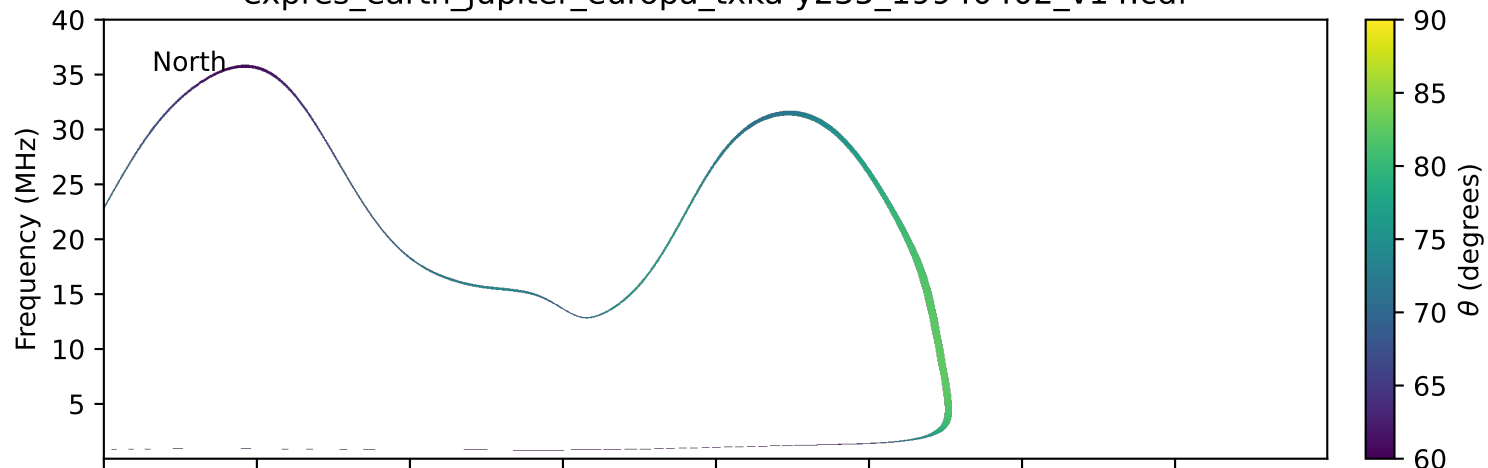
expres_earth_jupiter_europa_txka-y235_19940402_v14.cdf
