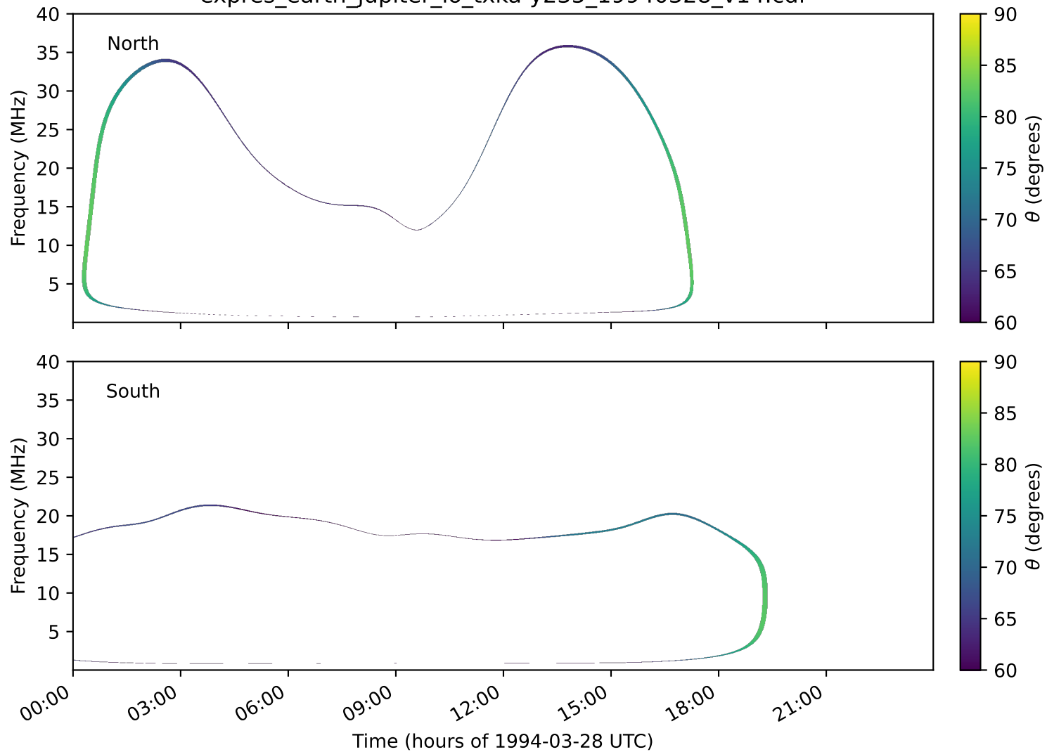
expres_earth_jupiter_io_txka-y235_19940328_v14.cdf
