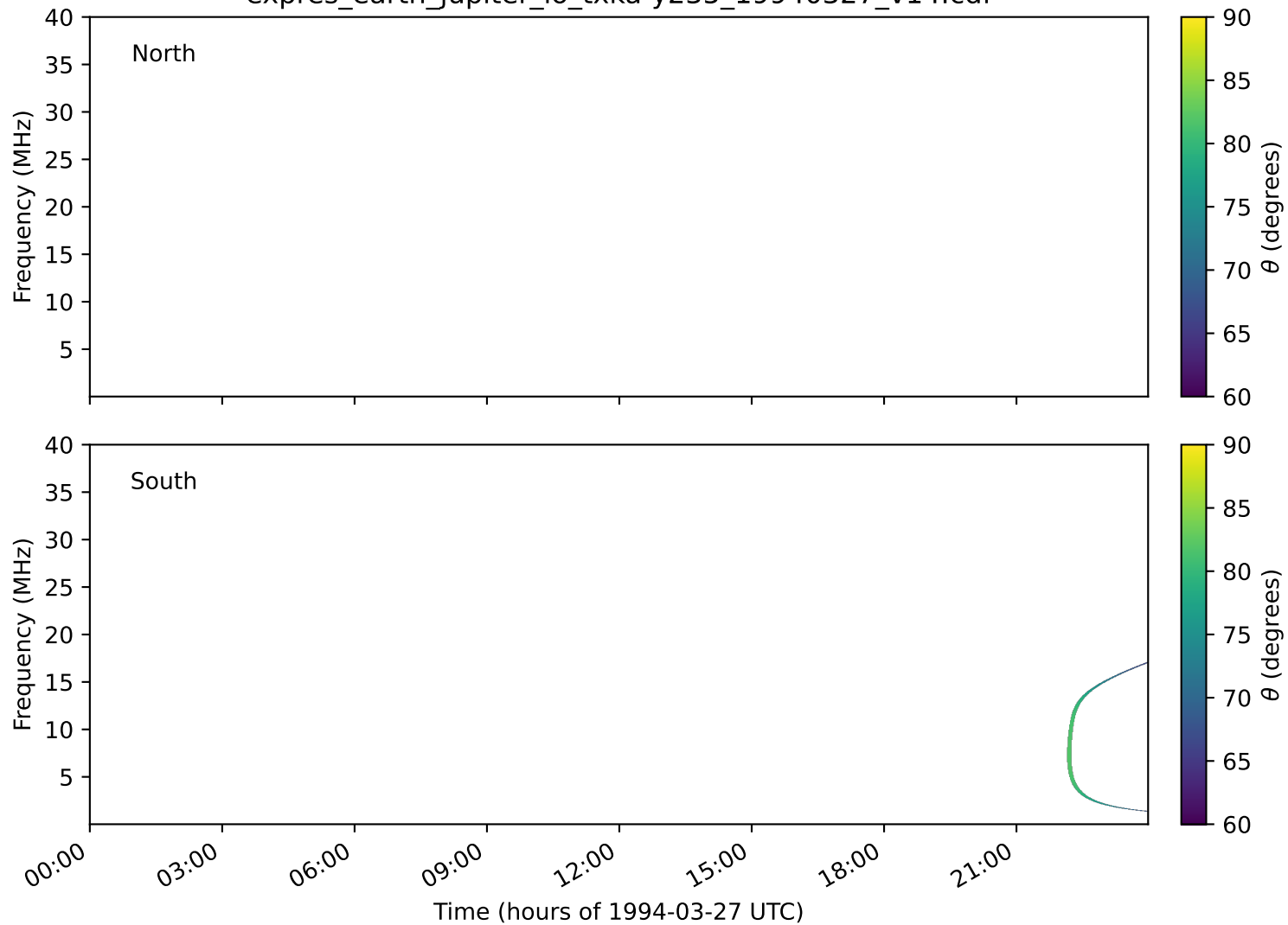
expres_earth_jupiter_io_txka-y235_19940327_v14.cdf
