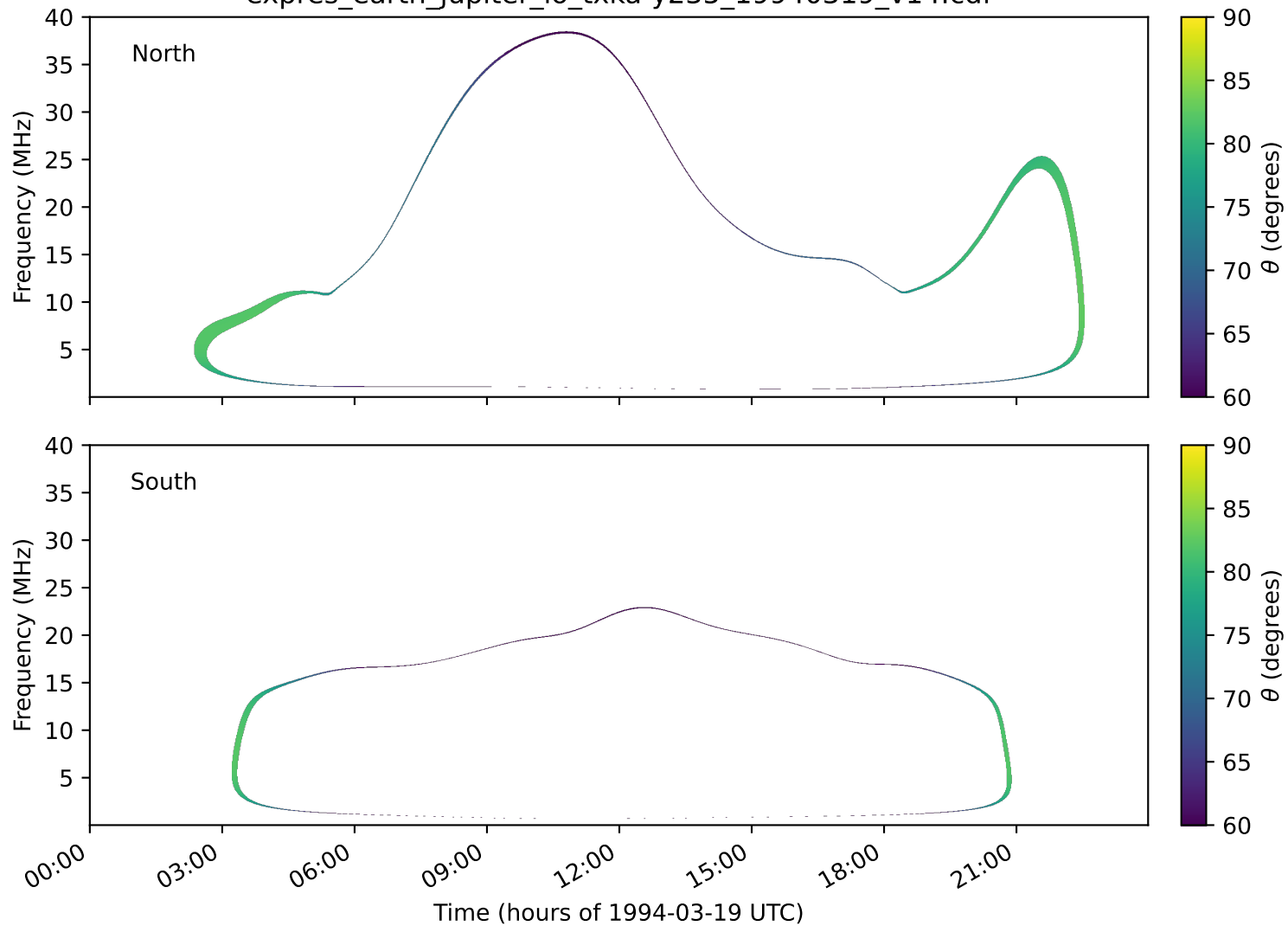
expres_earth_jupiter_io_txka-y235_19940319_v14.cdf
