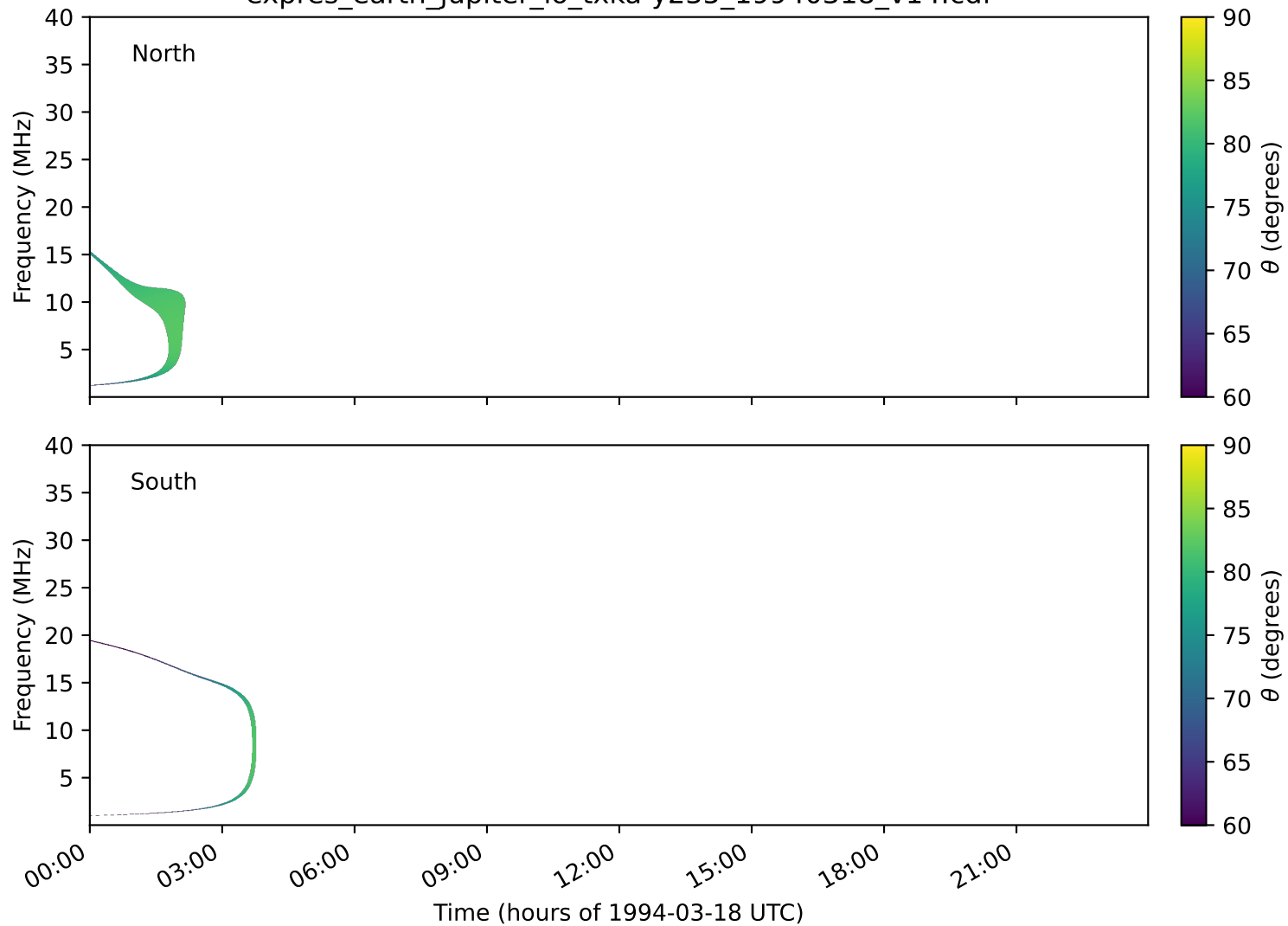
expres_earth_jupiter_io_txka-y235_19940318_v14.cdf
