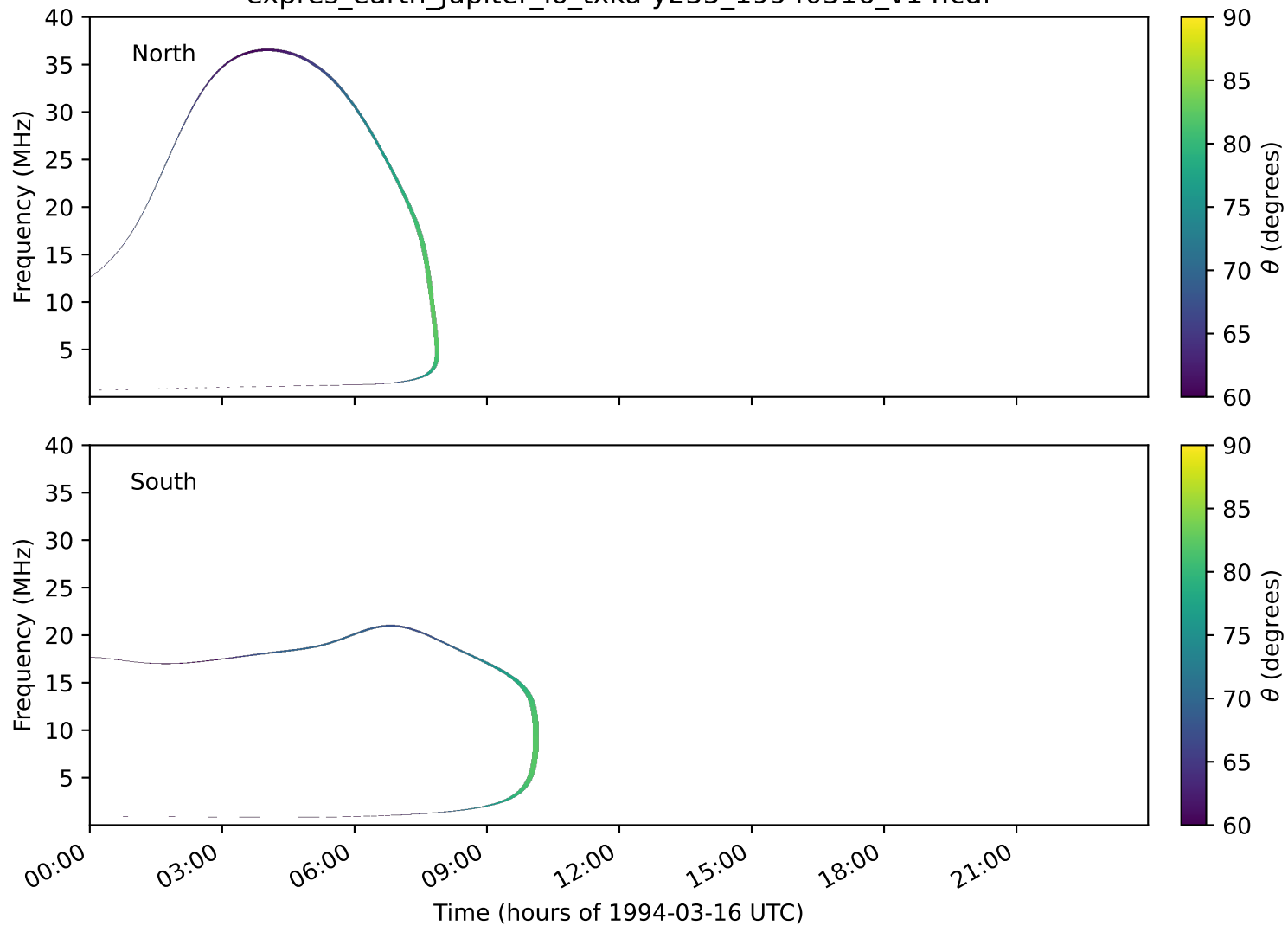
expres_earth_jupiter_io_txka-y235_19940316_v14.cdf
