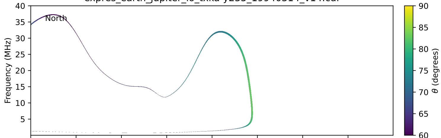
expres_earth_jupiter_io_txka-y235_19940314_v14.cdf
