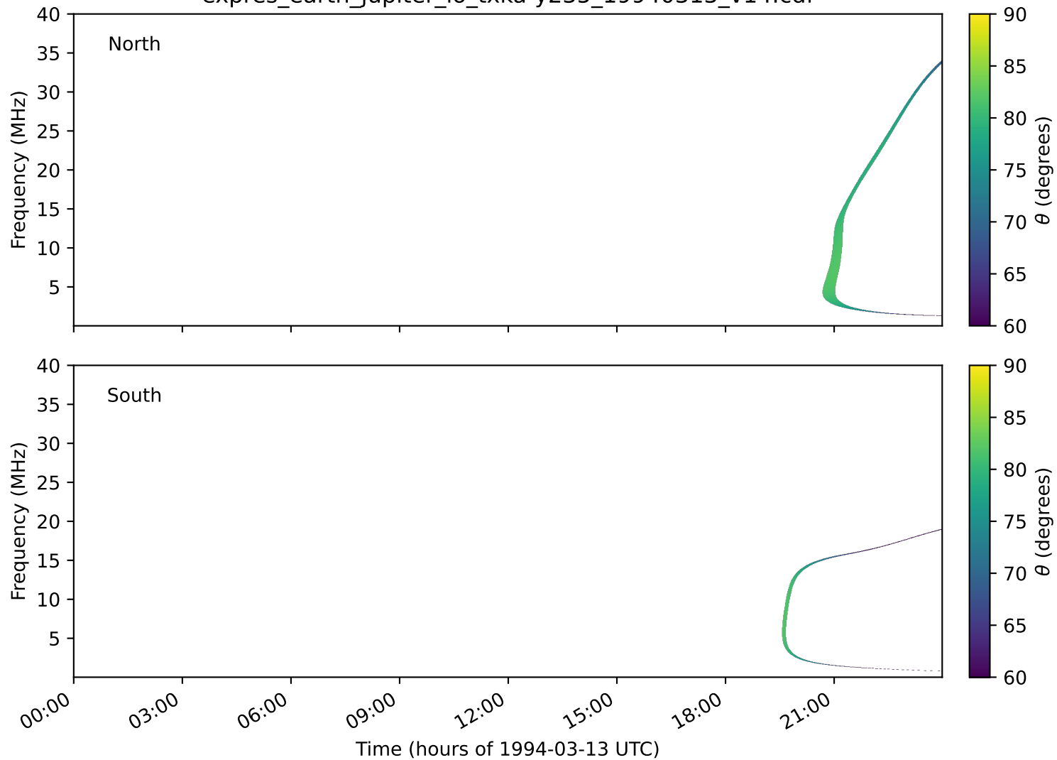
expres_earth_jupiter_io_txka-y235_19940313_v14.cdf
