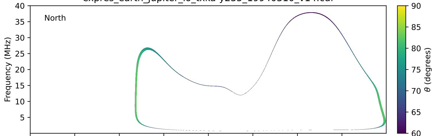
expres_earth_jupiter_io_txka-y235_19940310_v14.cdf
