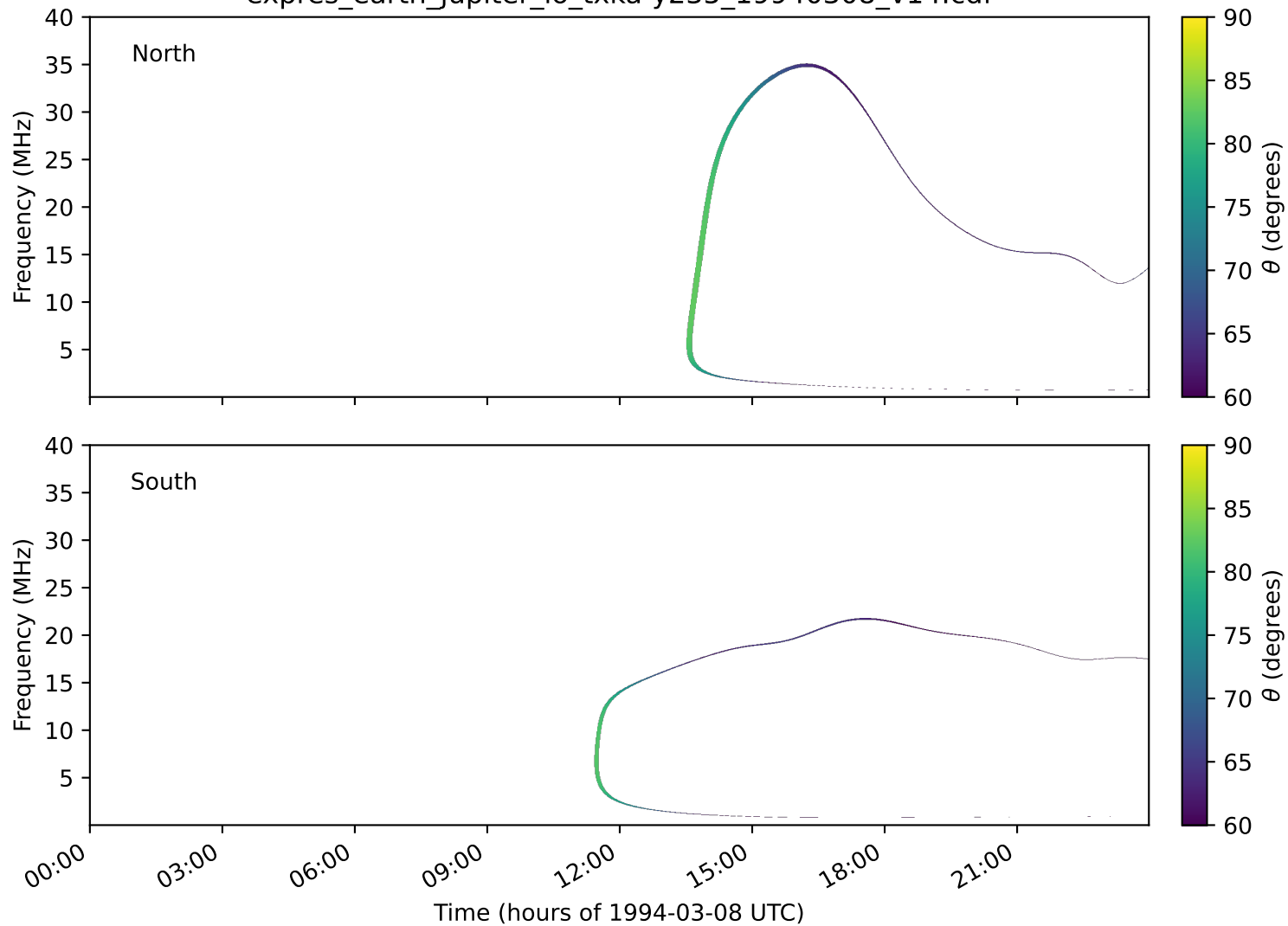
expres_earth_jupiter_io_txka-y235_19940308_v14.cdf
