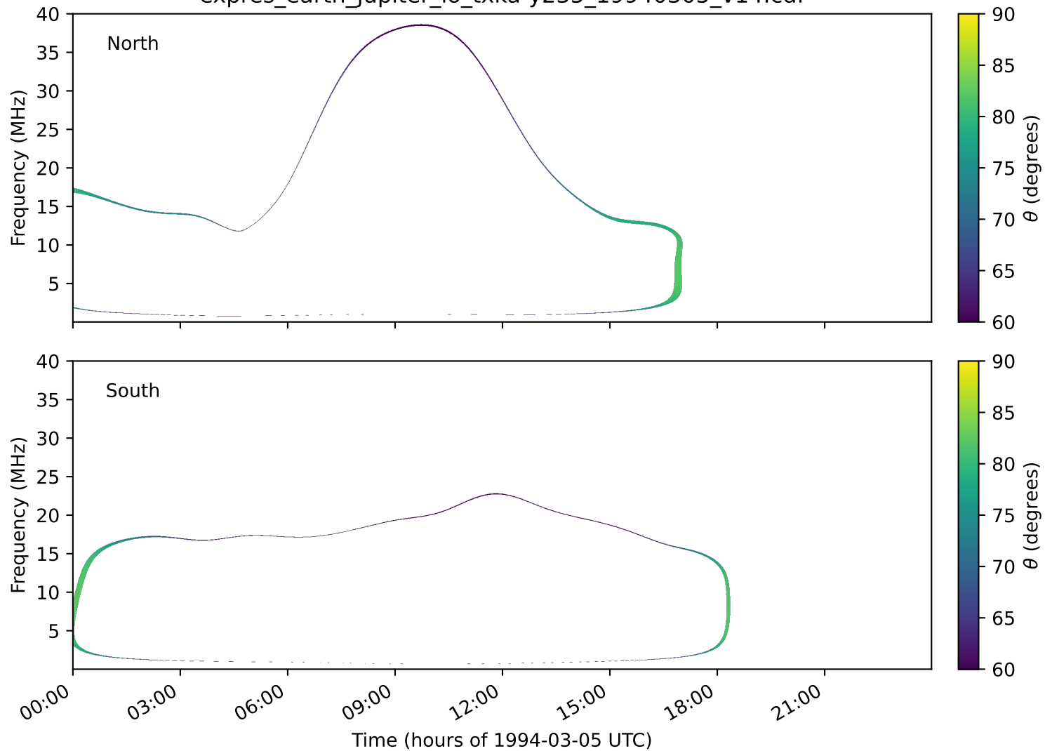
expres_earth_jupiter_io_txka-y235_19940305_v14.cdf
