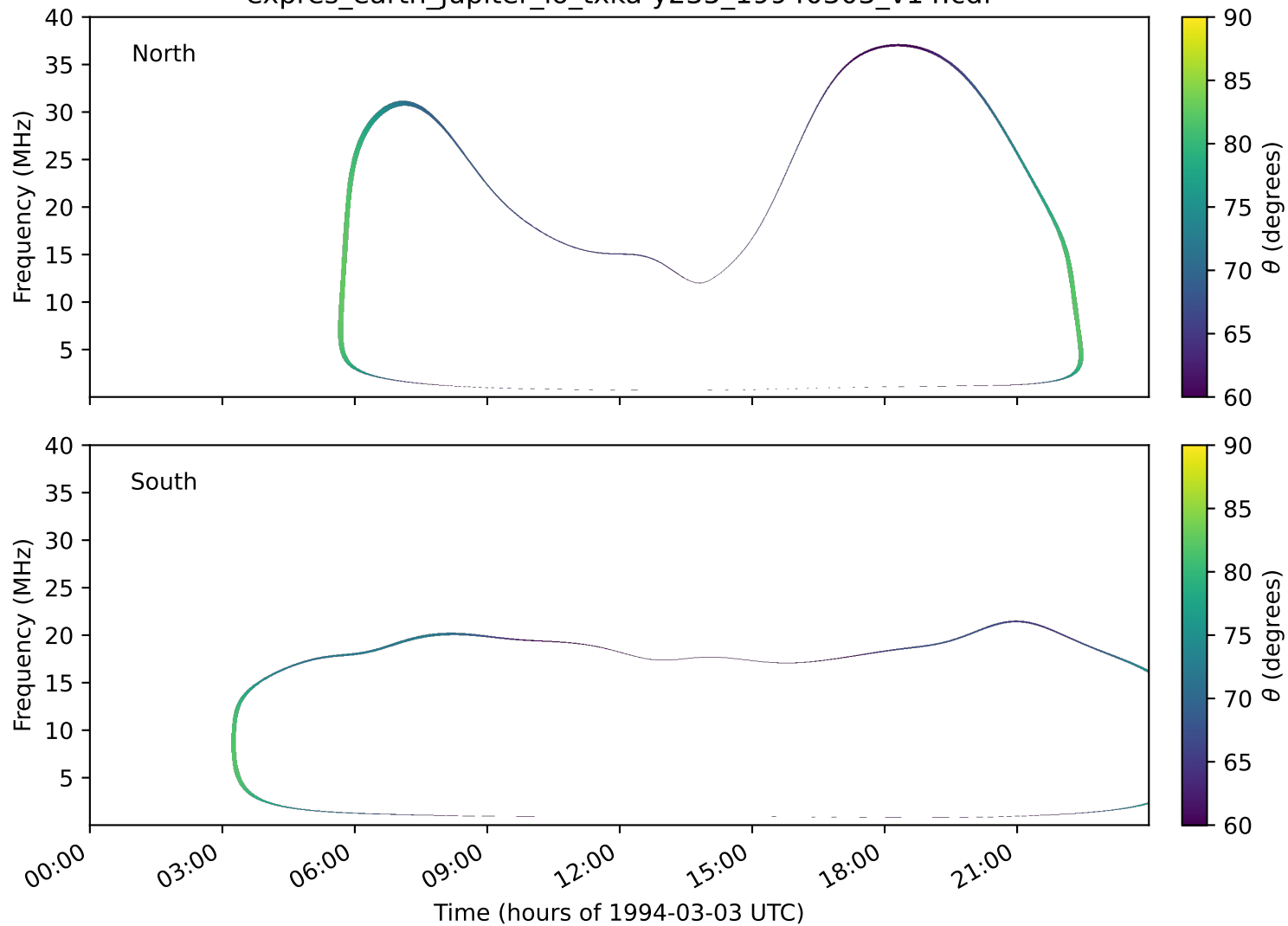
expres_earth_jupiter_io_txka-y235_19940303_v14.cdf
