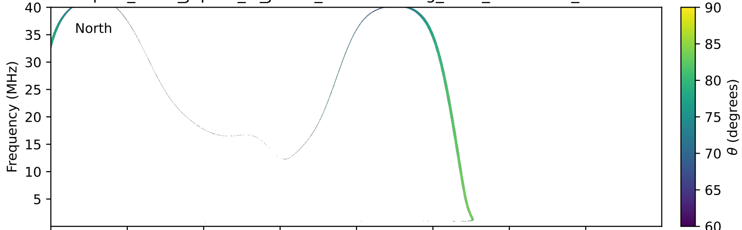
expres_earth_jupiter_io_jrm33_lossc-wid1deg_3kev_19940321_v11.cdf
