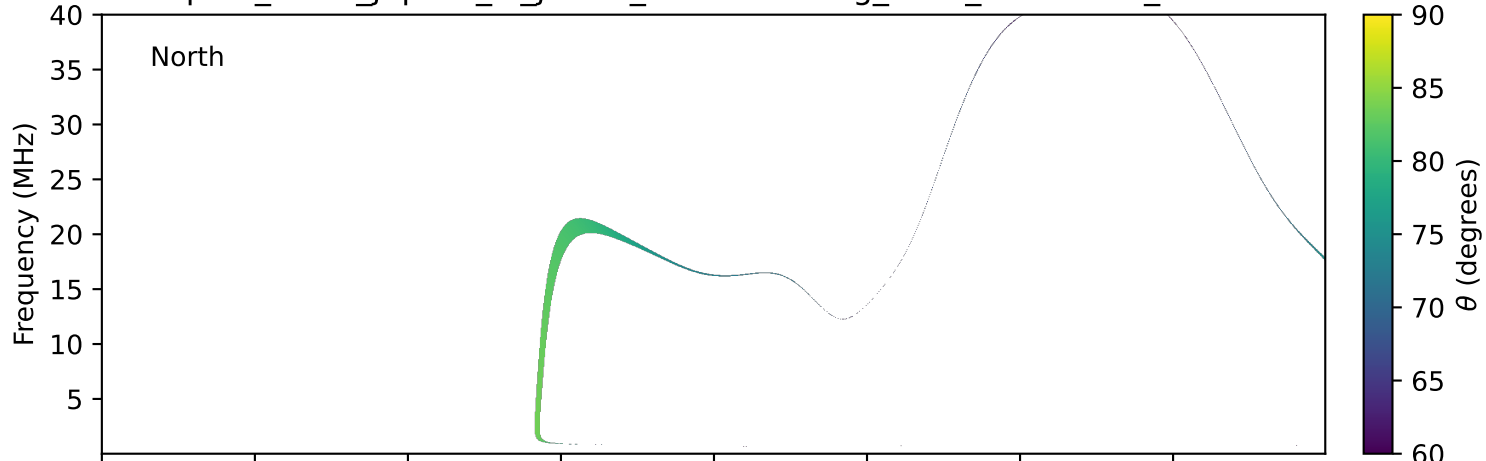
expres_earth_jupiter_io_jrm33_lossc-wid1deg_3kev_19940317_v11.cdf
