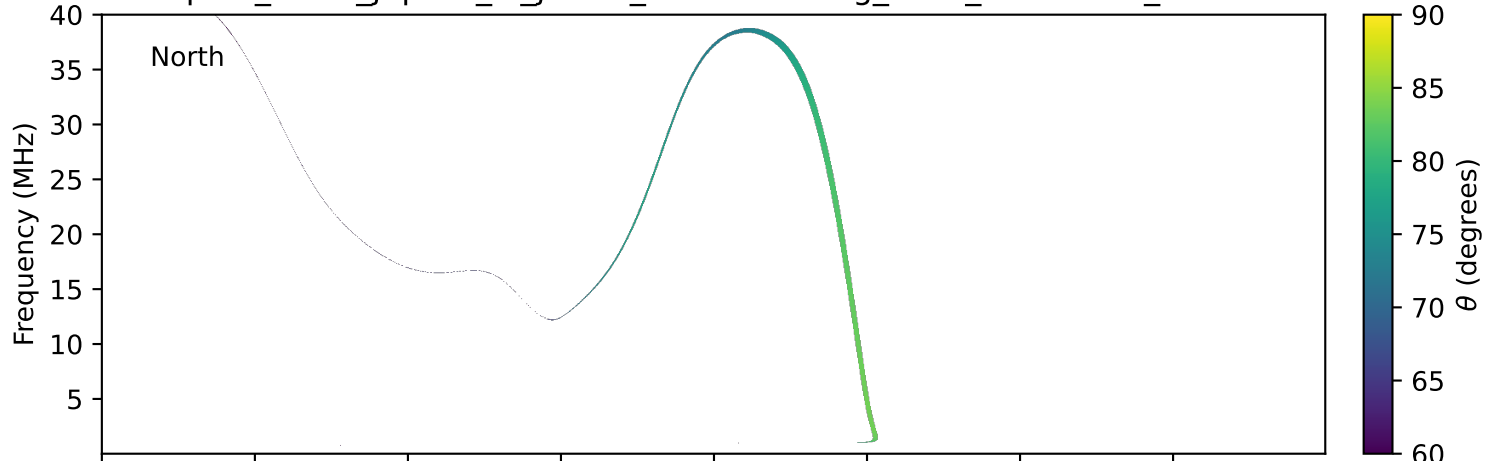
expres_earth_jupiter_io_jrm33_lossc-wid1deg_3kev_19940314_v11.cdf
