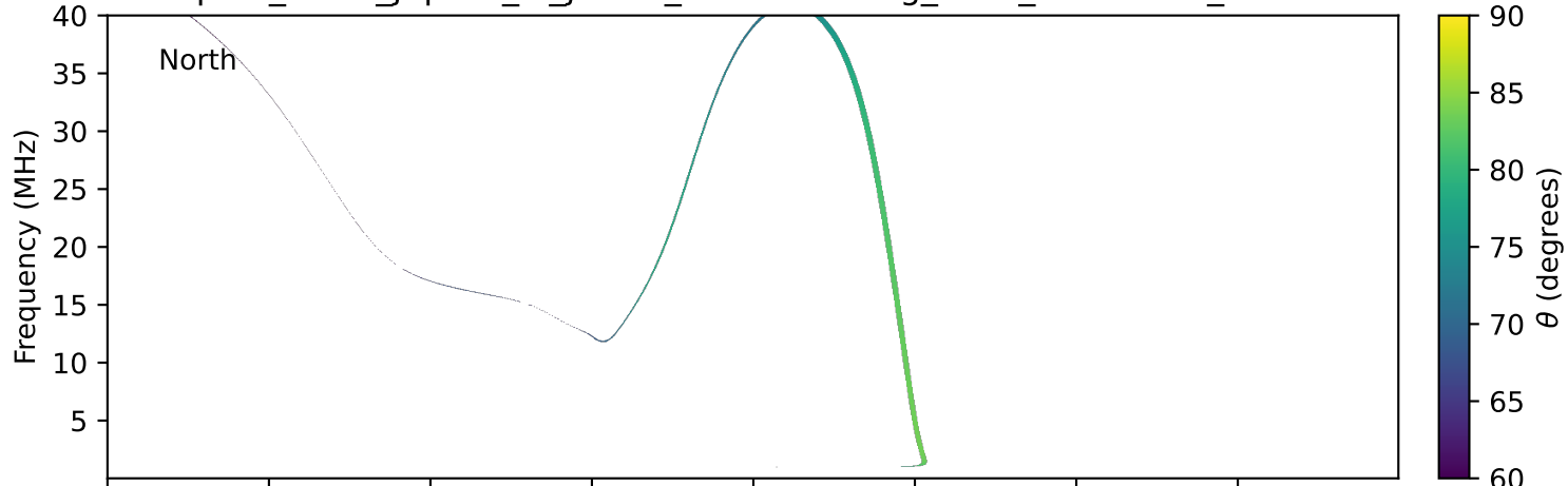
expres_earth_jupiter_io_jrm09_lossc-wid1deg_3kev_19940314_v11.cdf
