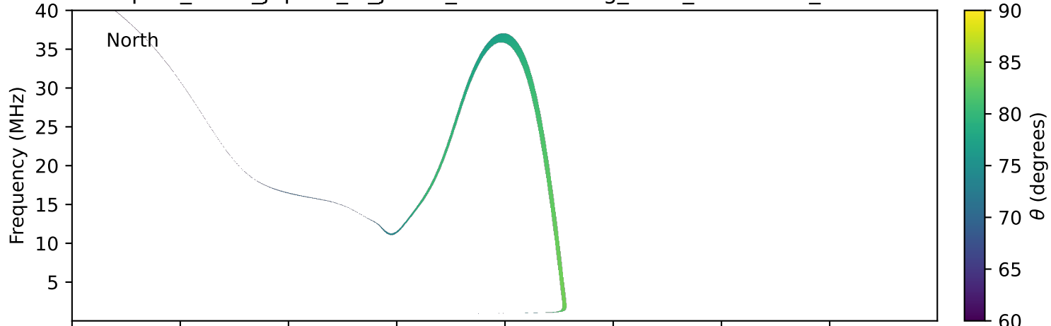
expres_earth_jupiter_io_jrm09_lossc-wid1deg_3kev_19940307_v11.cdf
