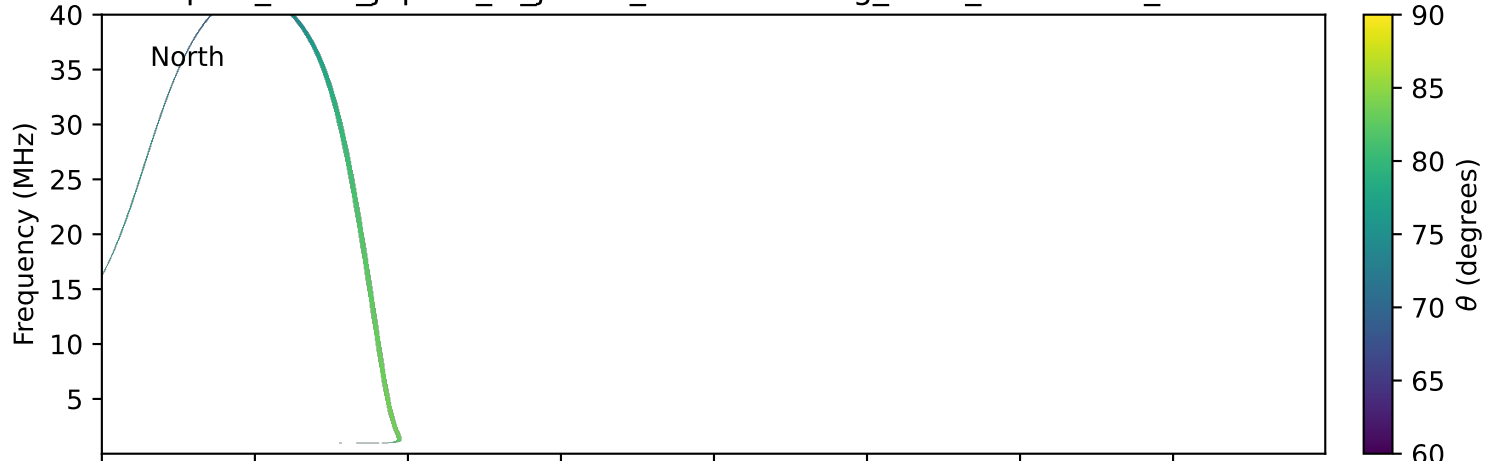
expres_earth_jupiter_io_jrm09_lossc-wid1deg_3kev_19940302_v11.cdf
