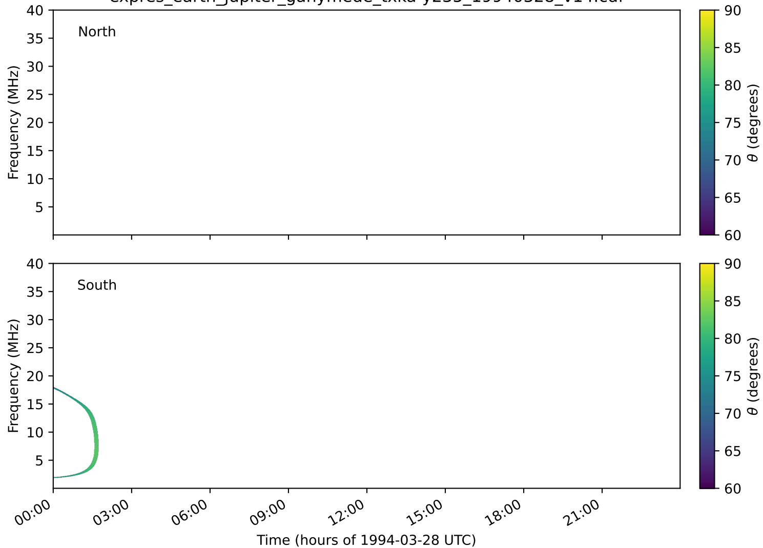
expres_earth_jupiter_ganymede_txka-y235_19940328_v14.cdf
