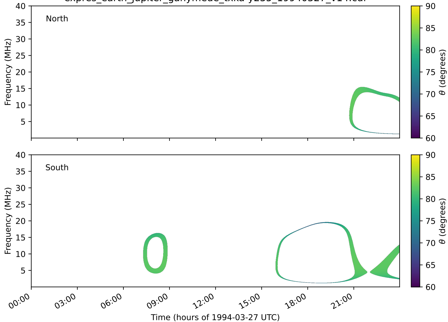
expres_earth_jupiter_ganymede_txka-y235_19940327_v14.cdf
