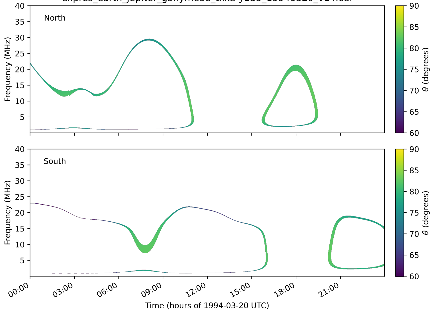
expres_earth_jupiter_ganymede_txka-y235_19940320_v14.cdf
