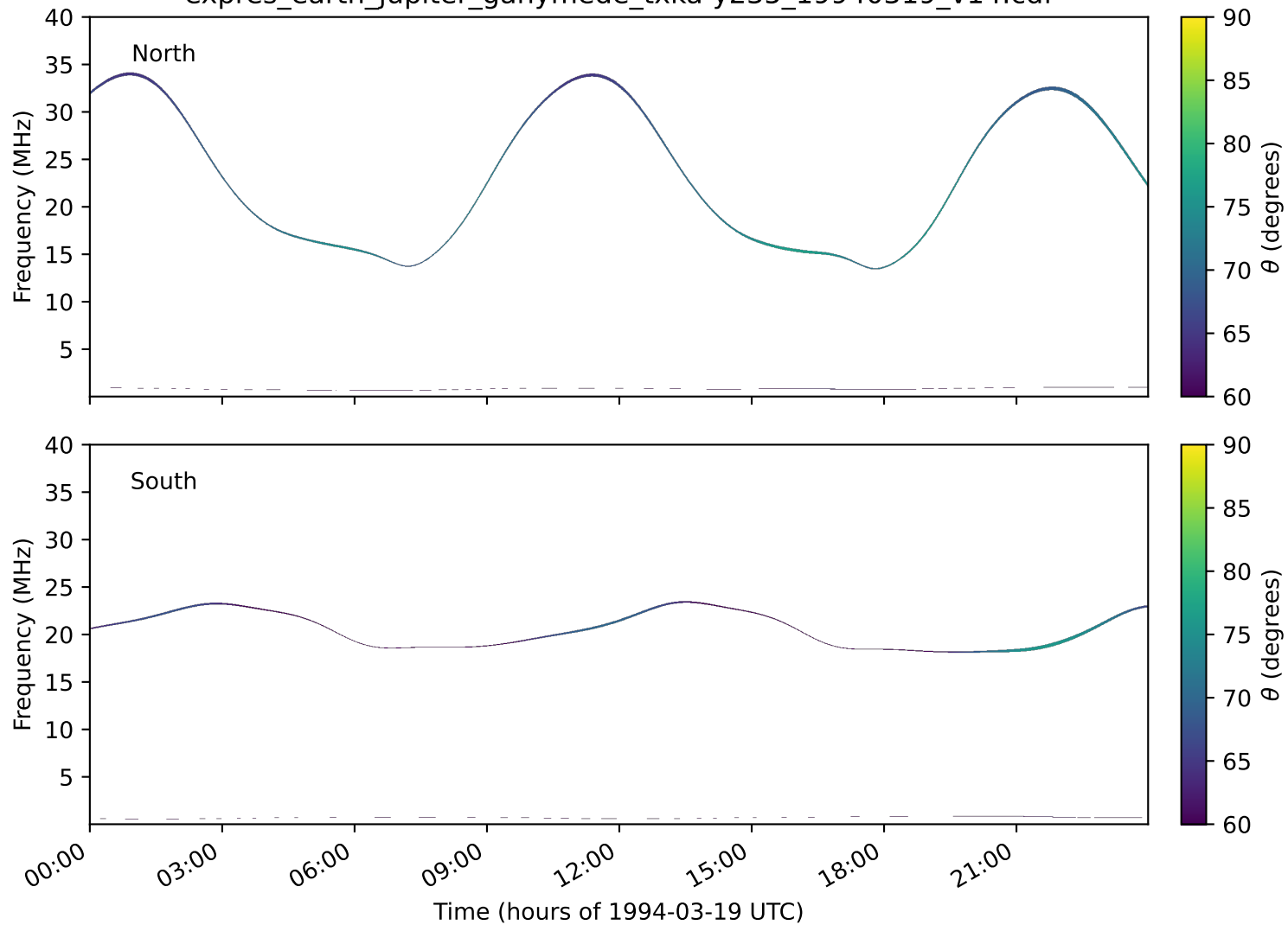
expres_earth_jupiter_ganymede_txka-y235_19940319_v14.cdf
