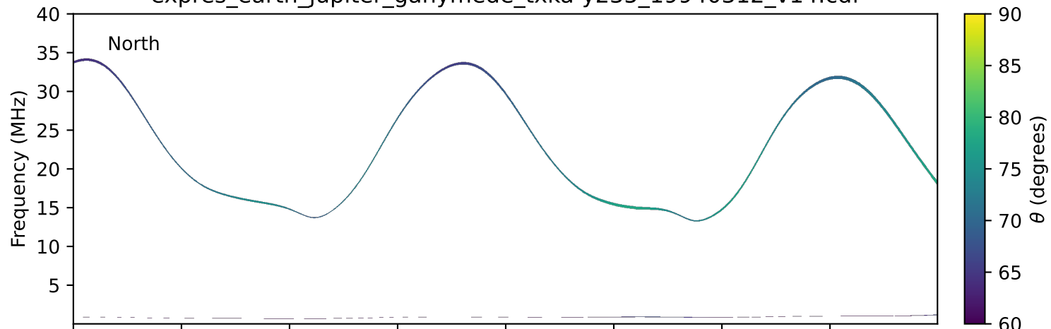
expres_earth_jupiter_ganymede_txka-y235_19940312_v14.cdf
